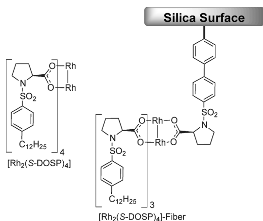
Scheme 1. Homogeneous [\text{Rh}_2(\text{S-DOSP})_4] and its immobilized analogue on silica. The other catalyst structures are shown in the Supporting Information.
